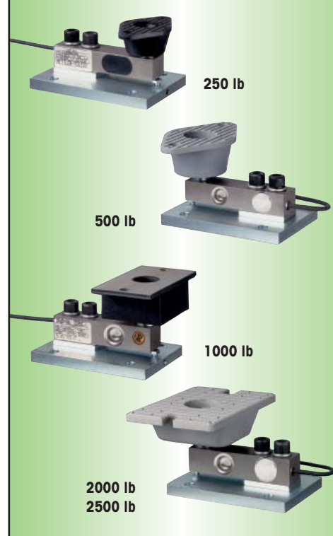
A variety of load cell configurations are available.
